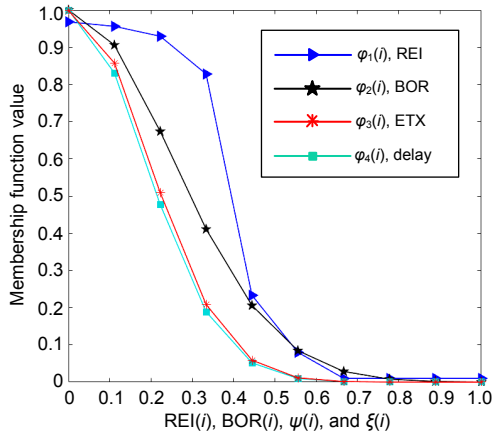
Fig. 6 Membership function curves
