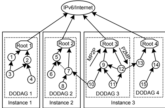
Fig. 1 RPL network topology with four DODAGs in three instances
